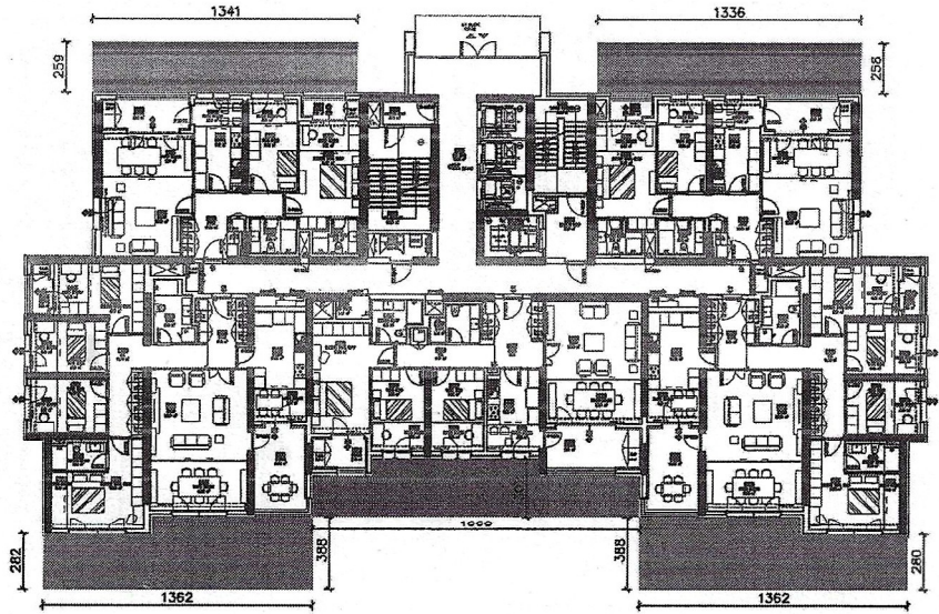
B3 BLOK ZEMİN KAT PLANI (0.00 (+55.15) kotu PLANI)
